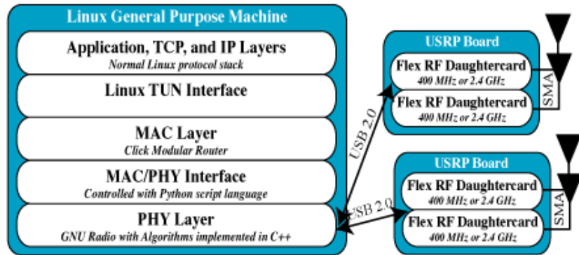
Figura 2–16: Diagrama a bloques de un nodo del sistema Hydra ( Wireless Networking Communications Group, 2007 )
